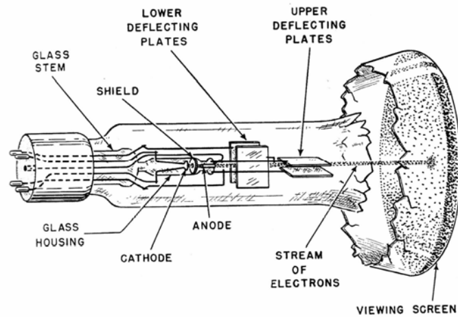
Fig. 2 - Drawing of the Johnson tube showing its electrode arrangement.
