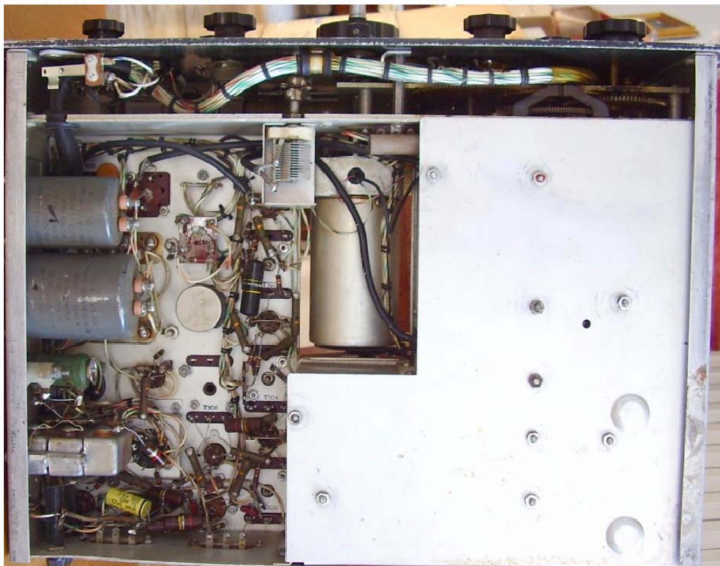
- A close-up view of the 70E-15 PTO and a bottom view of the chassis: a large shielding plate covers the RF and the variable IF coils.
