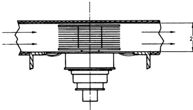
DETAILS OF AIR DUCT
