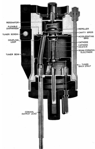
Cross-section of the 2K25 showing the internal structure. Click to enlarge.
