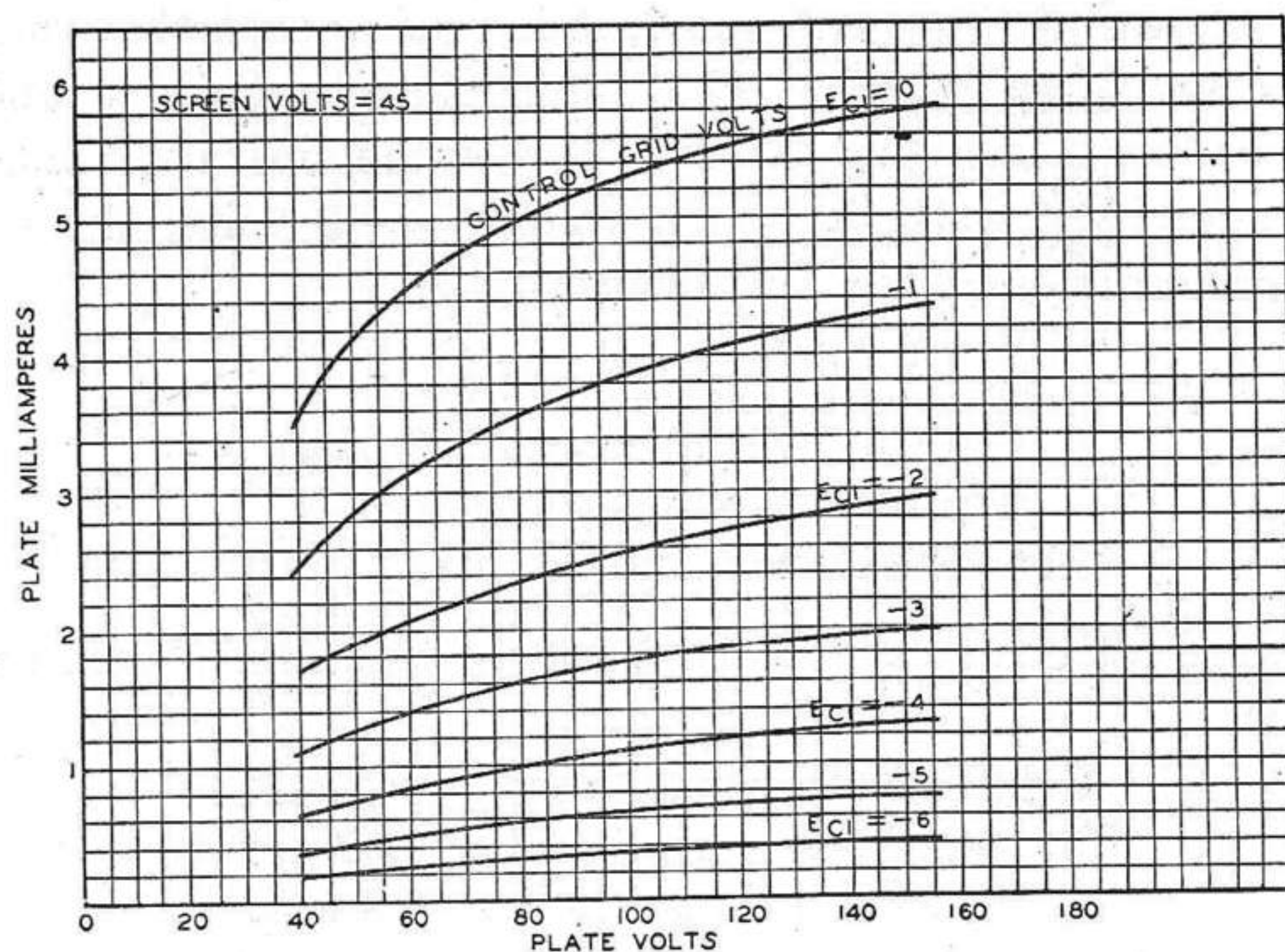
Fig. 7—Plate characteristics of the small screen-grid tube.
