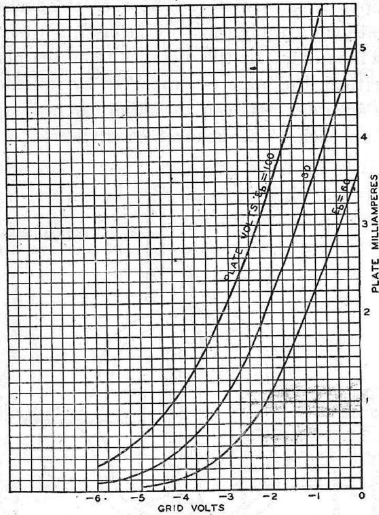
Fig. 5—Mutual characteristics of the small triode.
