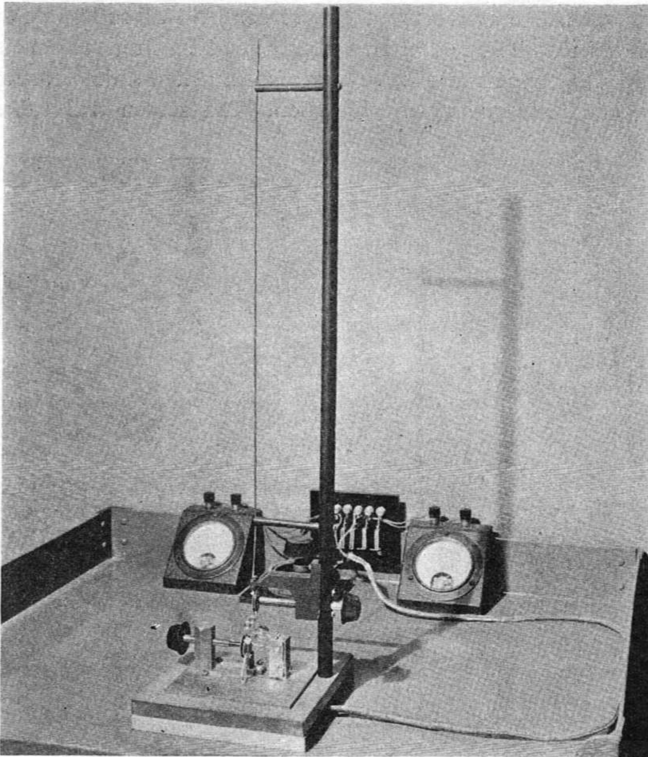
Fig. 14—Photograph of the 100-centimeter transmitter.
