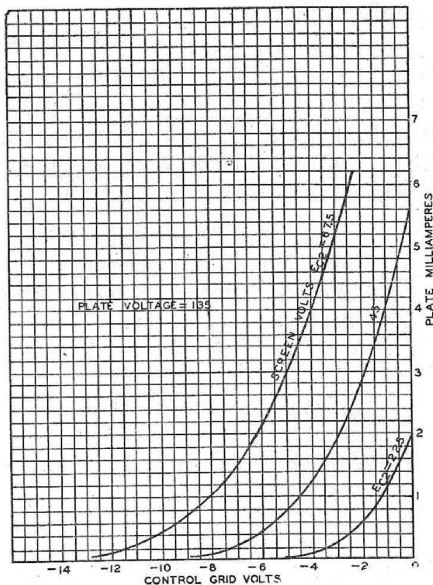
Fig. 8—Mutual characteristics of the small screen-grid tube.
