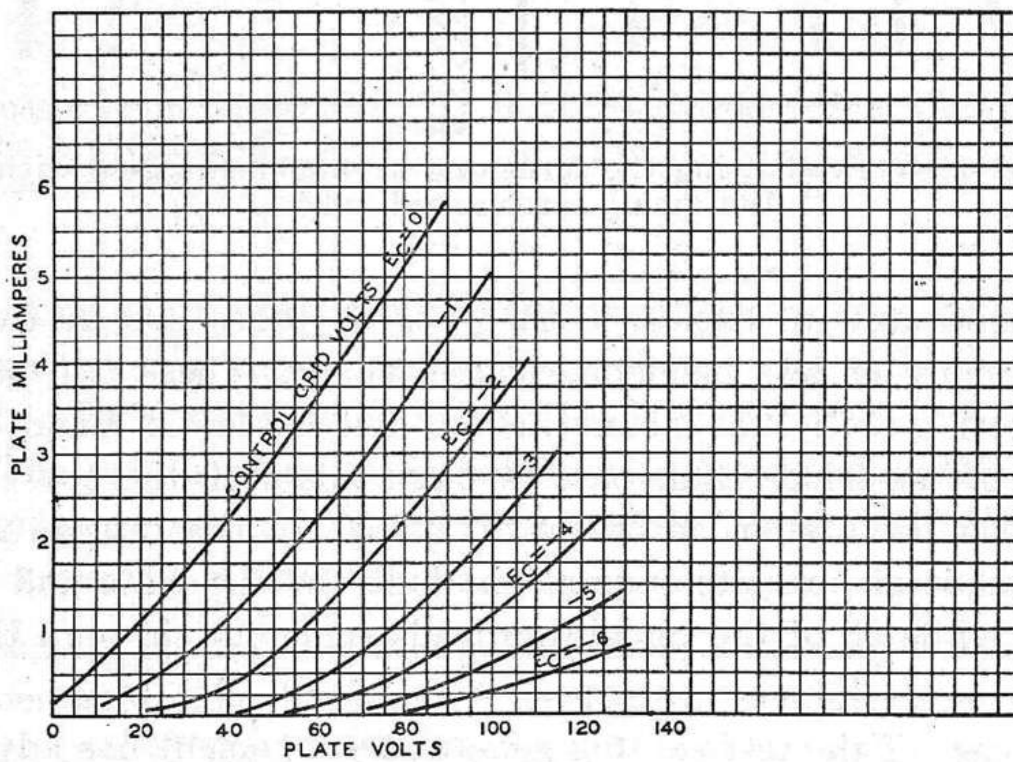
Fig. 6—Plate characteristics of the small triode.
