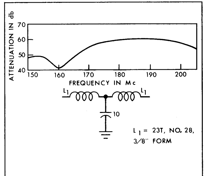
Figure 9-9. Low-pass filter useful for receiver protection
