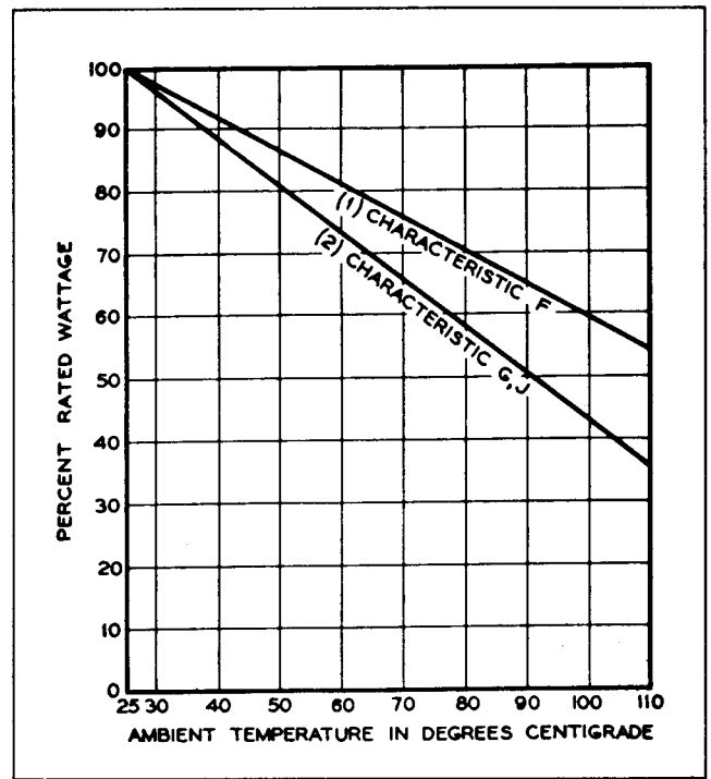
Figure 8-46. Derating curve for high-ambient temperatures
