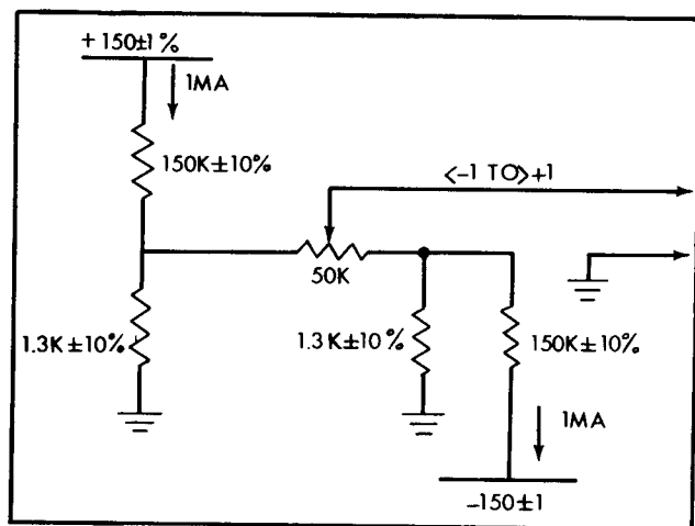
Figure 5-3. Voltage divider with resistors having tolerances of \pm 10 percent
