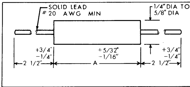
Figure 8-45. Axial wire lead terminal styles
