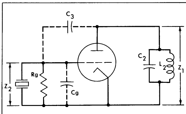
Figure 5-16. Miller oscillator
