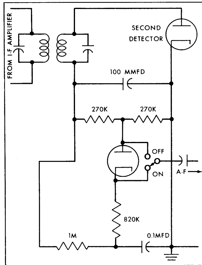
Figure 9-8. Series limiter
