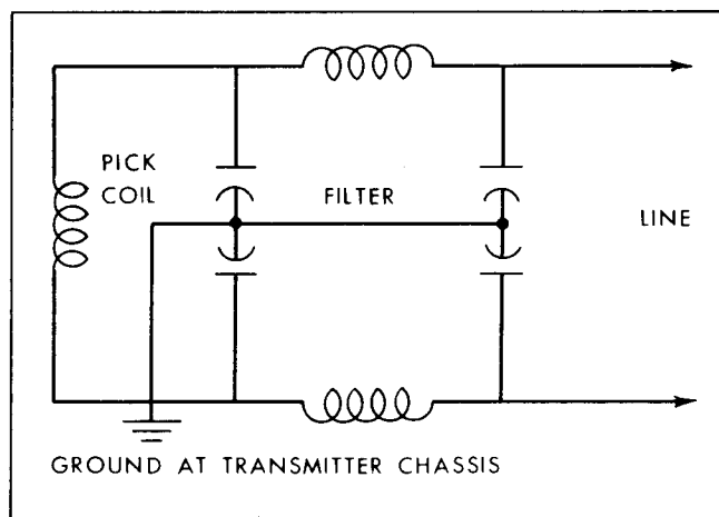
Figure 9-3. Capacitive harmonic coupling to a two-wire transmission line
