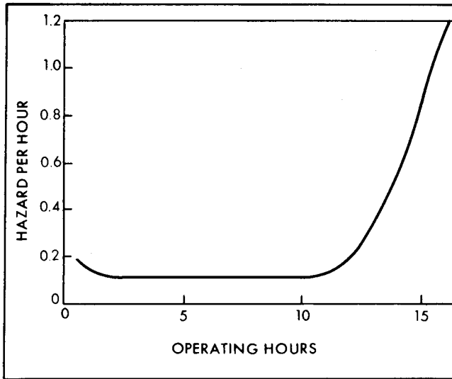
Figure 4-3. Typical hazard curve (corresponding to failure rate curve of Figure 4-1)
