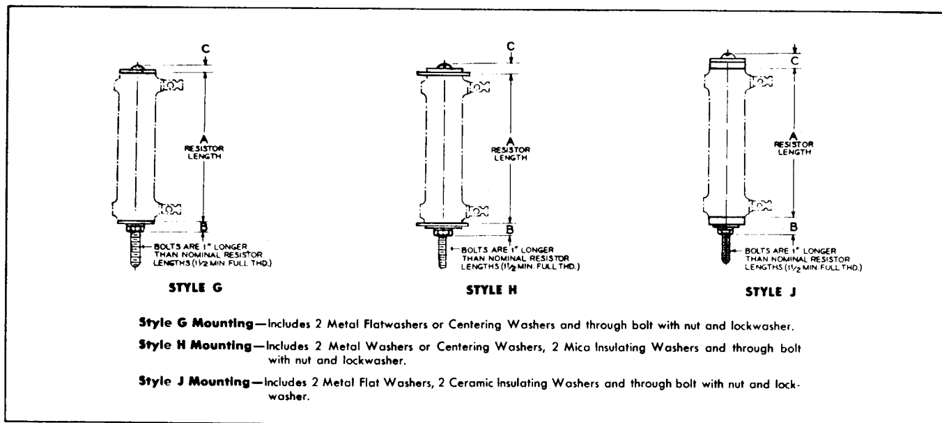
Figure 8-48. Through-bolt vertical mounting
