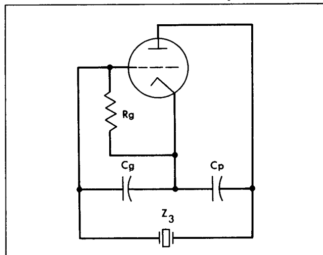
Figure 5-17. Pierce oscillator
