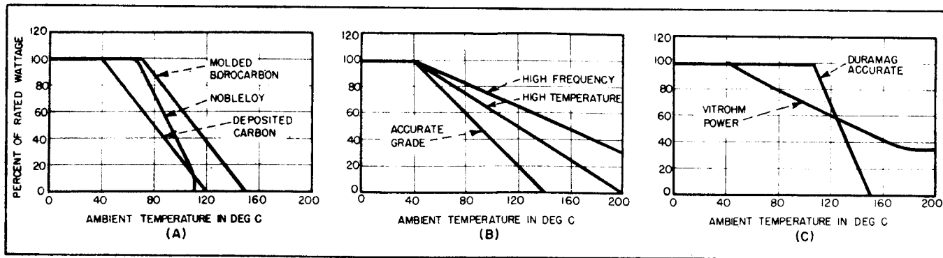
Figure 8-42. Derating curves for carbon-film resistors (A), film-on-glass (B), and wire-wound type (C)
