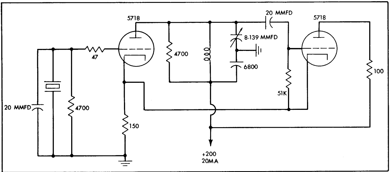
Figure 5-21. Regenerative feedback Miller oscillator
