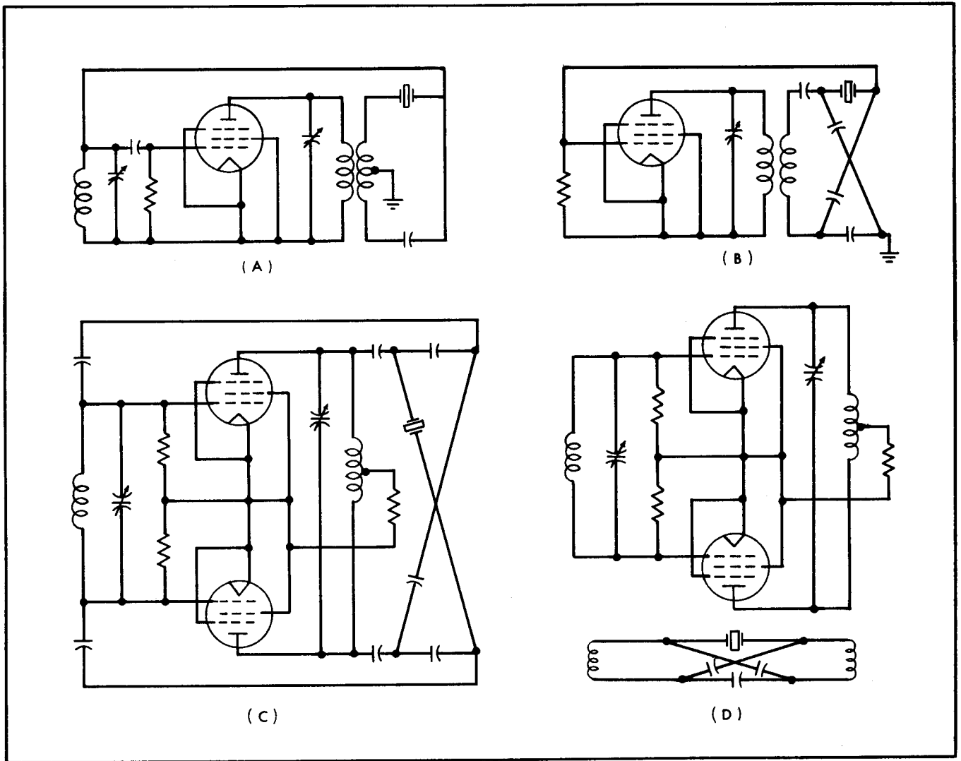
Figure 5-20. Elementary oscillators of the capacitance-bridge type, for very high frequencies
