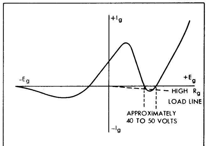
Figure 8-29. Typical curve of total grid current
