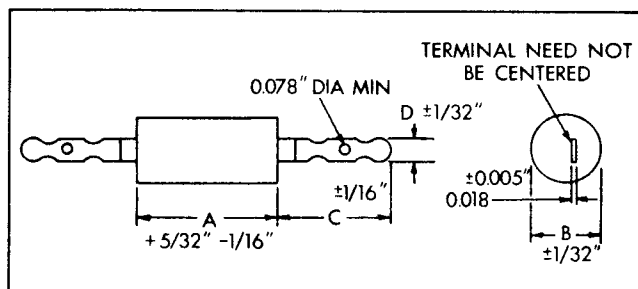
Figure 8-44. Axial lug terminal styles
