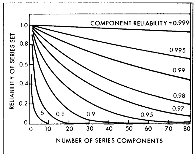
Figure 4-4. Reliability of " n " series components of equal reliability
