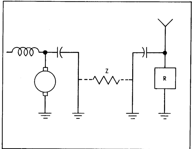
Figure 9-12. Unwanted motor noise coupled to circuit
