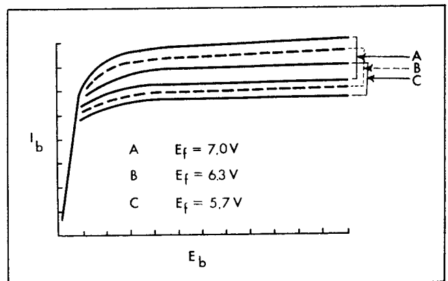
Figure 8-9. Pentode plate characteristics — Effects of variations of E_f
