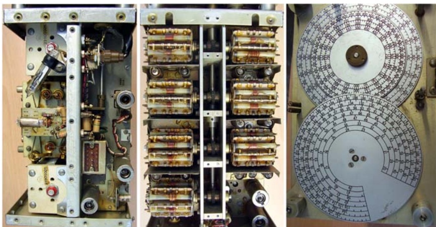
- Three views of the RF deck removed from the chassis.
