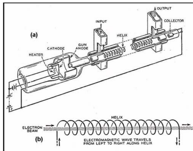
Fig. 1.38 – The TWT in the figure has the electron gun on the left. The generated electron beam travels to the collector through the helix, terminated at both sides by short coupling antennas. The beam is then captured by the collector at the extreme right. The signal propagates in the helix in the same direction of the electrons at approximately the same velocity, as in the draft 1.38(b).
