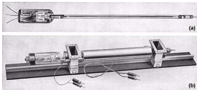
Fig 1.40 – Early TWT prototypes at Bell Telephone. The lower tube is mounted into the waveguide input and output transitions, with the focusing coil between them.
