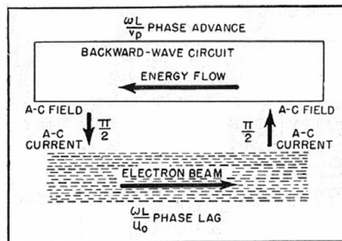
Fig. 1.44 – The RF field is propagated in the transmission line from right to left, with a phase velocity slightly lower than the velocity of the electron beam, that moves from left to right. On the left energy is transferred from the line to the beam, on the right it returns back to the line, each transfer adding 90-degree phase lag.
