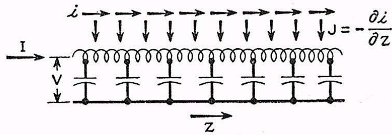
Fig. 1.39 – Model of the TWT proposed by Pierce. The helix is here represented as a lumped-constants line and the signal moves forward in the direction z ; successive arrows, indicated as i , represent the convection current of the electron beam. The current ( J ) impressed from electrons to the propagating signal is given by the relation on the right.
