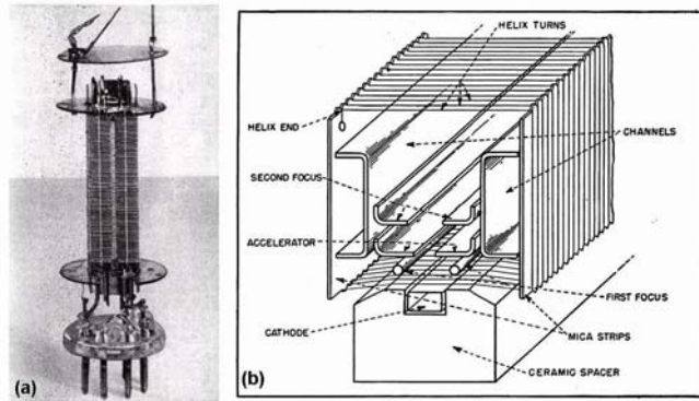
Fig. 1.41 – In the miniature TWT signal enters from the base, travels through the helix and is available on the top. Right, a cross-section view of electrodes. The tube operated in a magnetic field. Electronics, October 1951.
