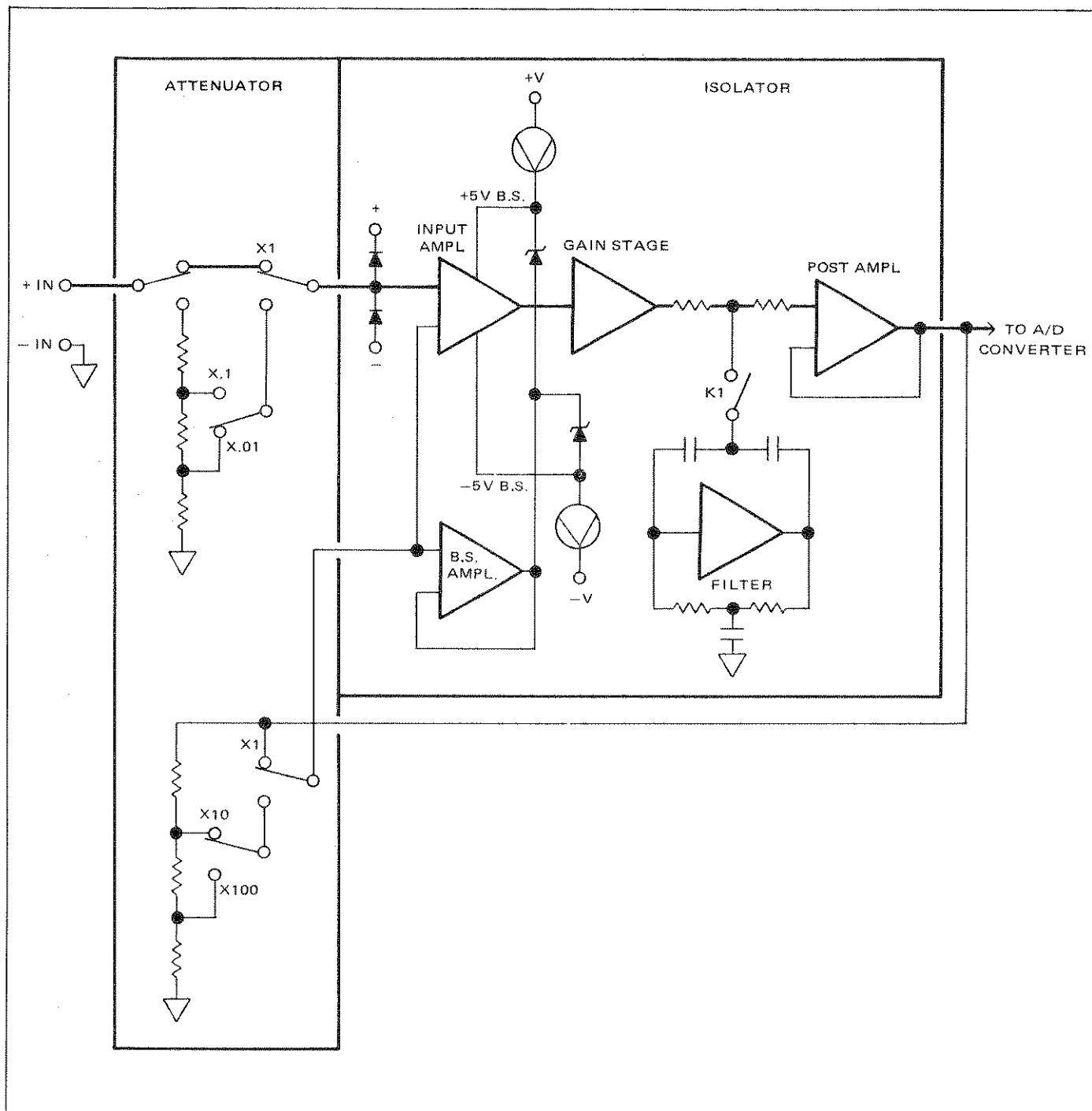
Figure 4.10 - Attenuator/Isolator DC
