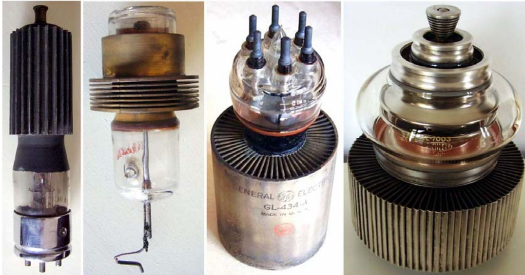
Fig. 17 - Power tubes with air-cooled external anode made of copper sealed to the glass bulb. Radiating fins are brazed to the copper surface.
